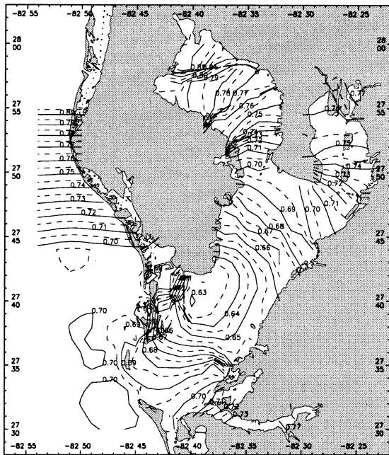
Figure B.1. MHHW (m) relative to MLLW.
