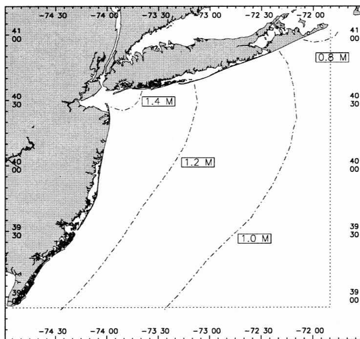
Figure 6.1. New York Bight and mean tide range (dash-dot lines, with range value in meters) from the MESA data. The offshore boundaries of the project are shown as dotted lines.
