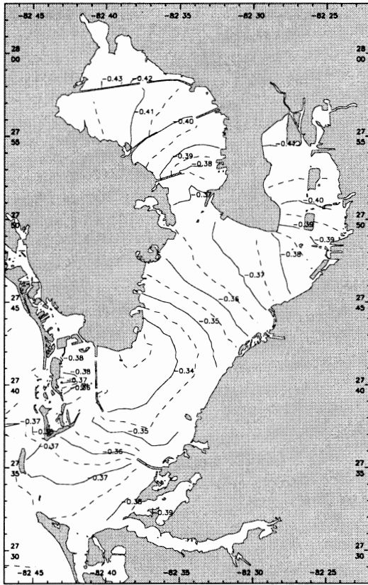
Figure 5.2a. The MSL-to-MLLW field generated by the hydrodynamic model.
