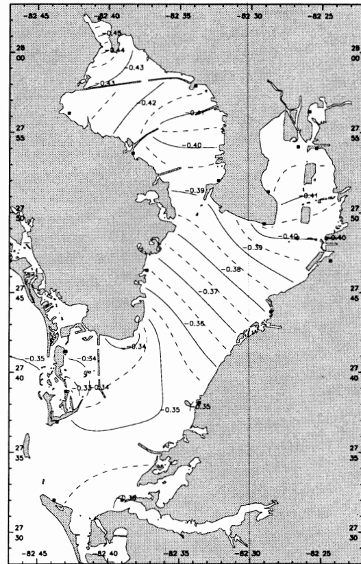
Figure 5.2b. The MSL-to-MLLW field generated by spatial interpolation.
