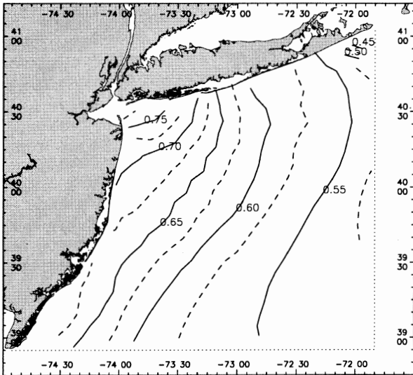
Figure E.1. The MHHW field (m).
