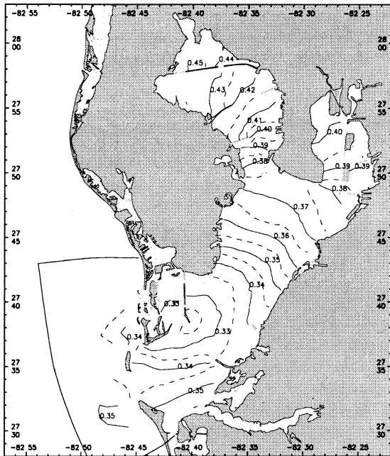
Figure A.1. MHHW.
