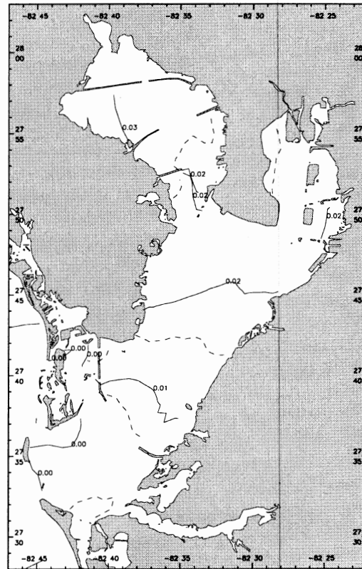
Figure 5.1b. MSL (m) from a 365-day model run.
