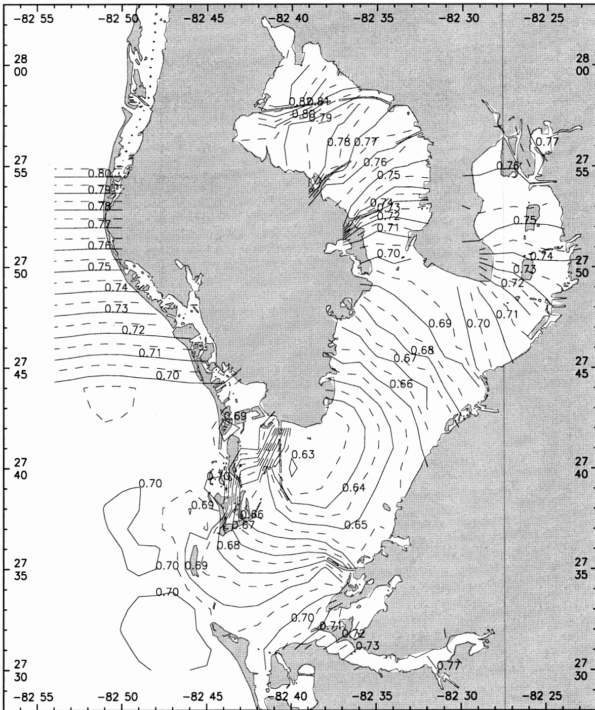
Figure 4.3. The region field of MHHW relative to MLLW (m).
