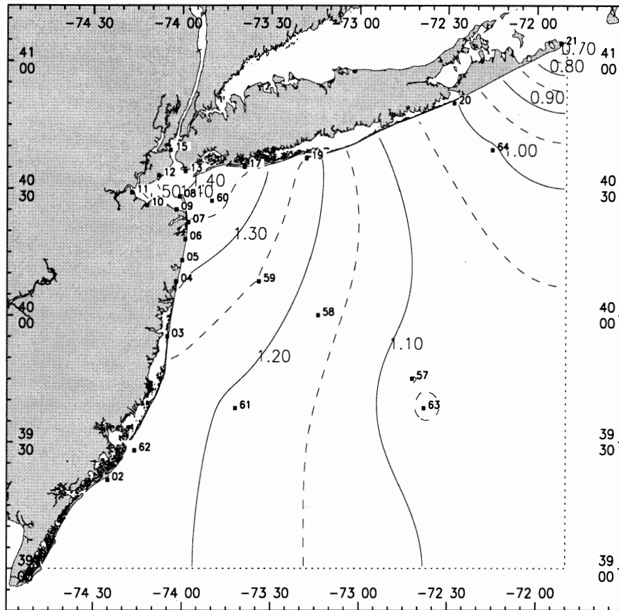
Figure 6.2. Mean tidal range as computed by the LE method. Numbered squares (see Appendix D for values) show the location of the MESA data used.
