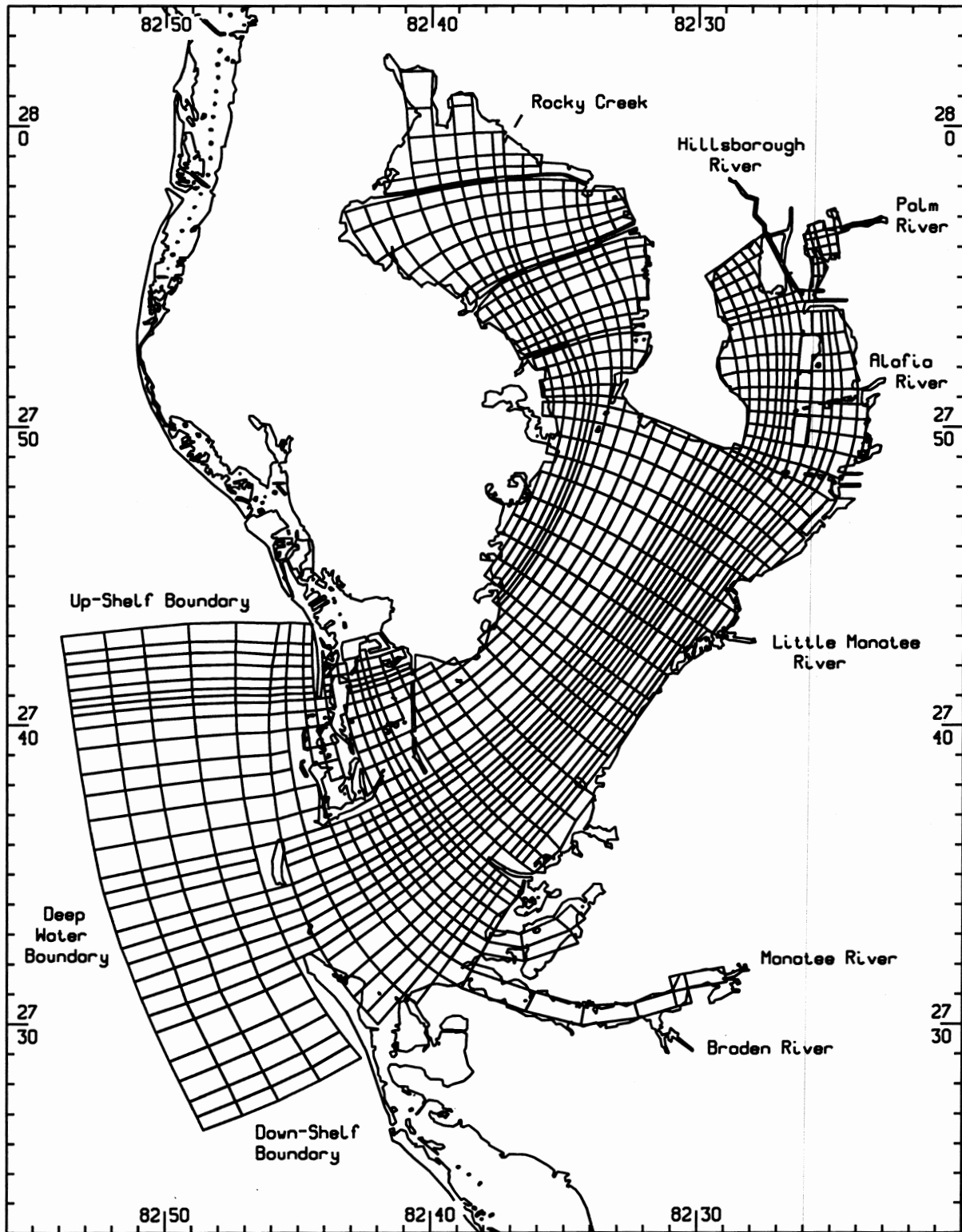
Figure 3.1. Grid used by the Tampa Bay numerical circulation model. Locations of the coastal boundaries and the rivers that provide fresh water are also shown.
