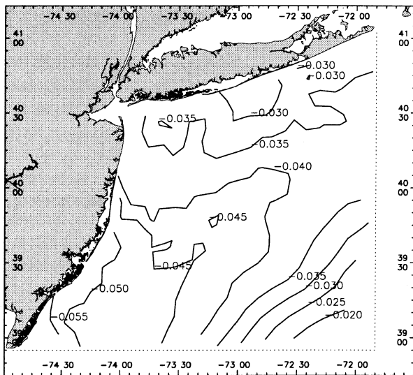
Figure E.7. The MTL field (m).
