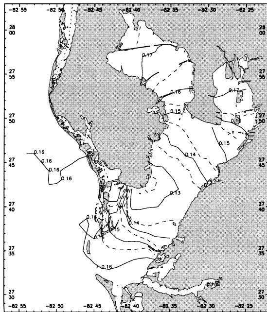
Figure B.3. MLW (m) relative to MLLW.
