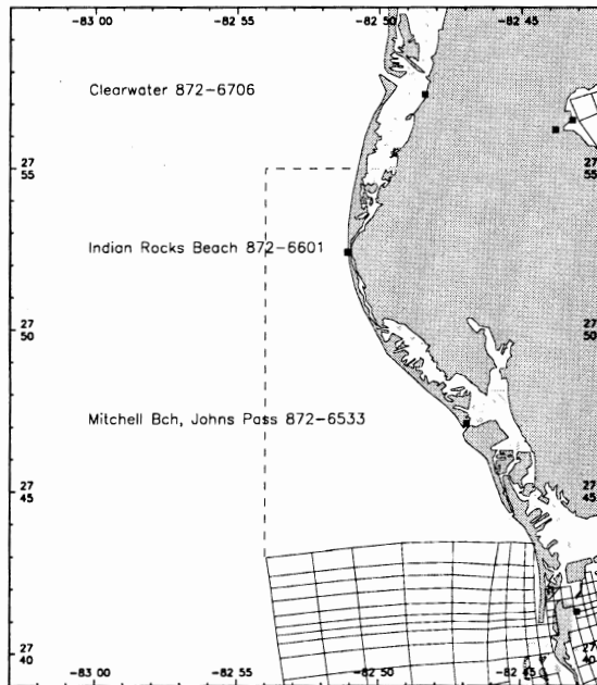
Figure 4.2. Region outside Tampa Bay where tidal datums were spatially-interpolated from gauge values and model values.
