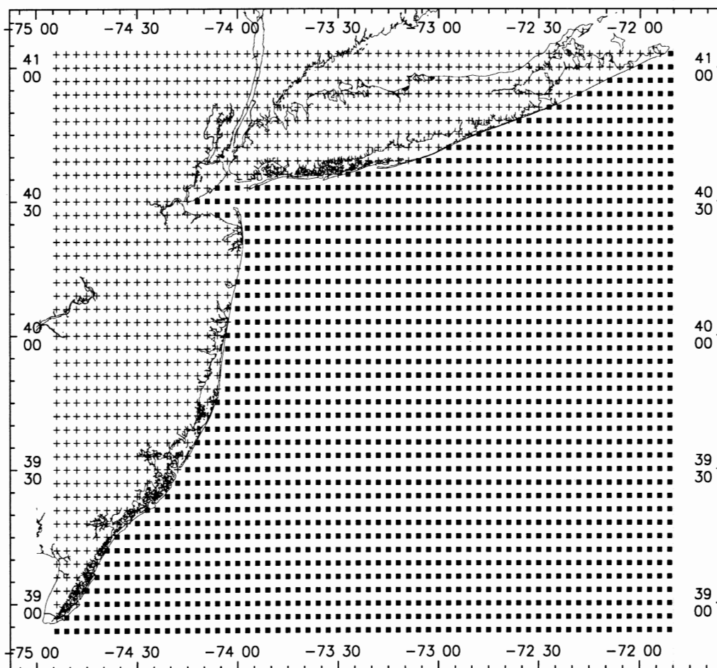
Figure 6.7. The datum transformation grid showing location of points used by VDatum. Filled squares show locations where datum transfer values are valid and locations denoted by a '+' hold only the default value.
