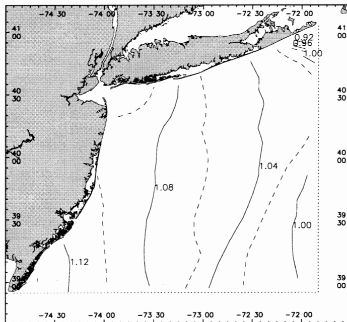
Figure 6.5. The tidal datum correction field, C(R, \phi, \lambda) .
