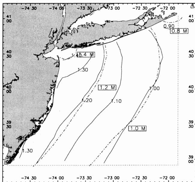
Figure 6.6. Modeled mean tide range (solid lines) after applying correction. The MESA data are dash-dot lines, with range values in boxes.
