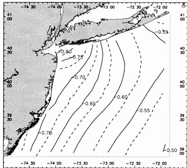
Figure E.4. The MLLW field (m).
