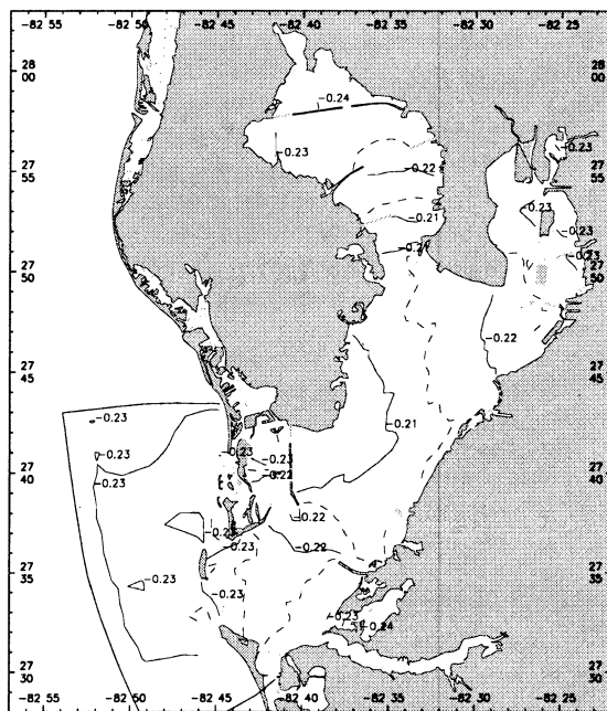
Figure A.4. MLW.
