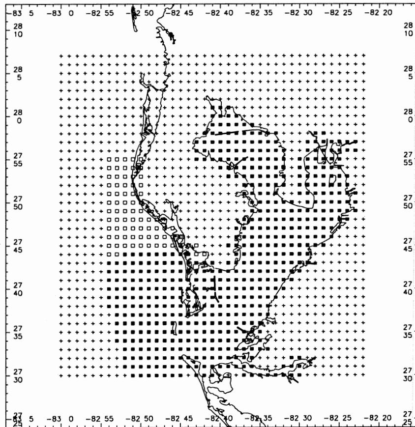
Figure 4.1. Locations of regional datum field grid points, with values created from the circulation model data (filled squares) and from interpolation of data based on observations (open squares). Points with default values are denoted by a plus sign. Spacing of nodes in each direction is 1 arc minute.
