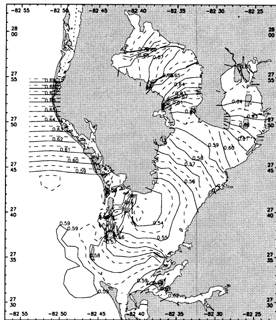
Figure B.2. MHW (m) relative to MLLW.
