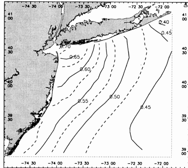
Figure E.2. The MHW field (m).
