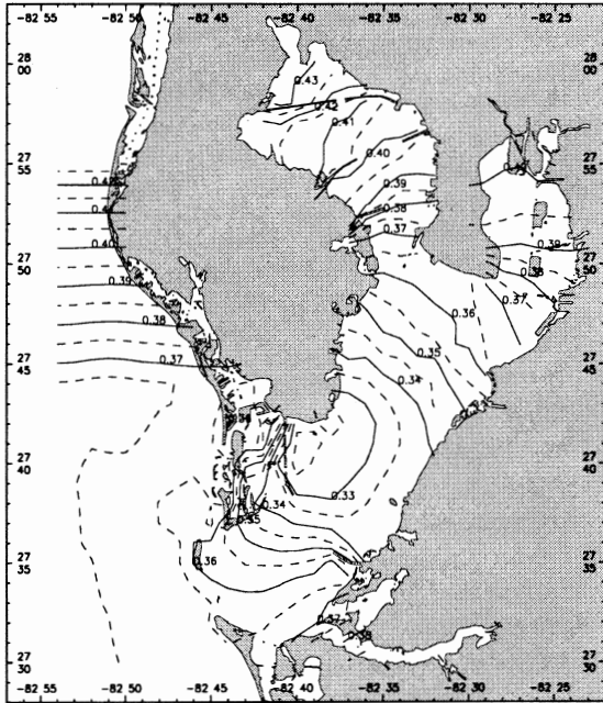
Figure B.6. MTL (m) relative to MLLW.
