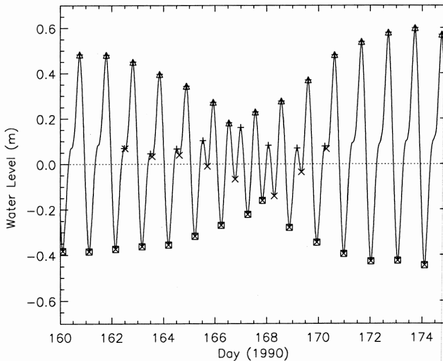
Figure 2.3. Portion of a modeled water level time series showing the selected higher high waters (triangle), high waters (“+”), low waters (“X”), and lower low waters (square).
