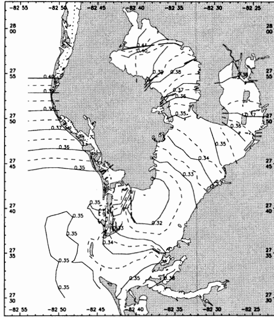
Figure B.6. DTL (m) relative to MLLW.
